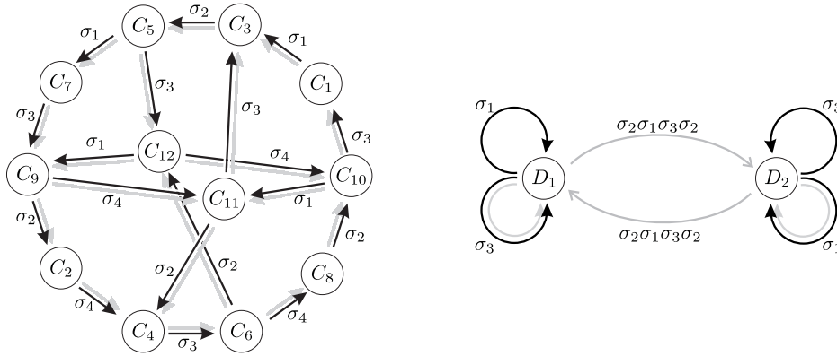
Figure 3. \Gamma_C and \Gamma_D .
