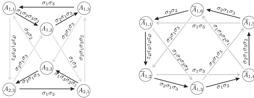
Figure 1. The graphs \Gamma_A and \Gamma_{A^{-1}} = \Gamma_{A^{-1}} .
