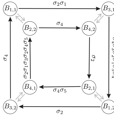
Figure 2. \Gamma_B .
