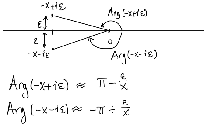
Figure 13: The jump discontinuity of \text{Log} along its branch cut.
