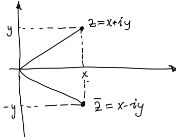
Figure 2: The geometric interpretation of complex conjugation.
