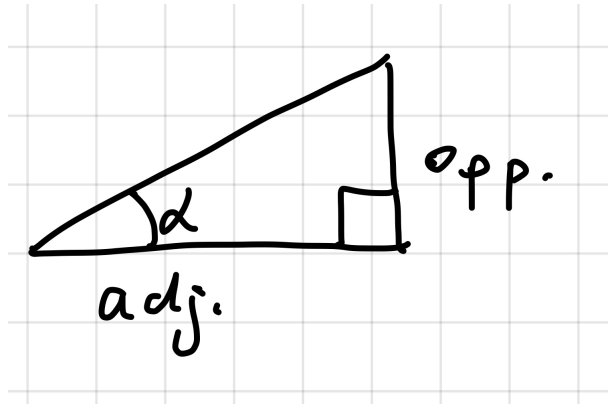
Figure 22: Tangent function.
