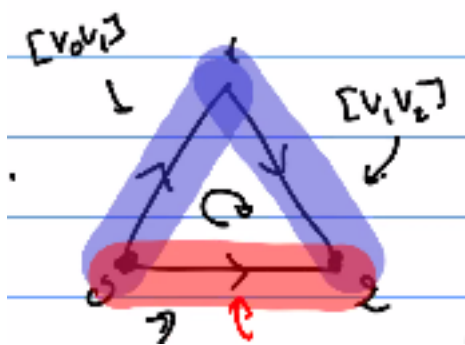
Figure 3.1: Simplicial orientations.
